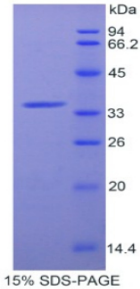
SDS-PAGE Image
