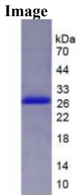
Figure. SDS-PAGE
