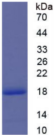
Figure. SDS-PAGE
