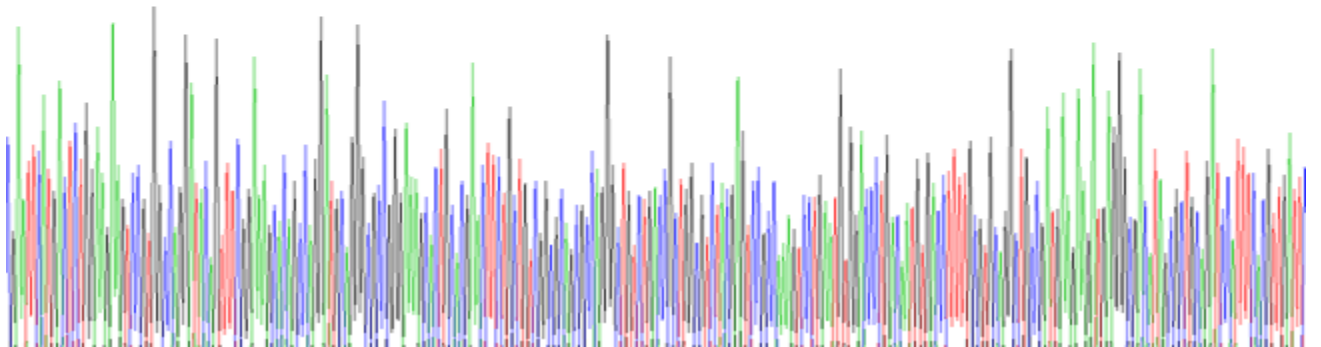
SDS-PAGE Image
