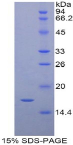
SDS-PAGE Image
