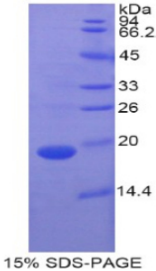
SDS-PAGE Image
