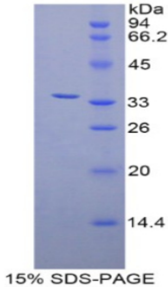
SDS-PAGE Image
