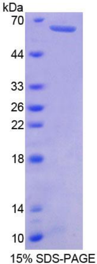
Figure. SDS-PAGE
