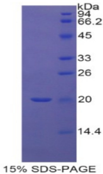
SDS-PAGE Image
