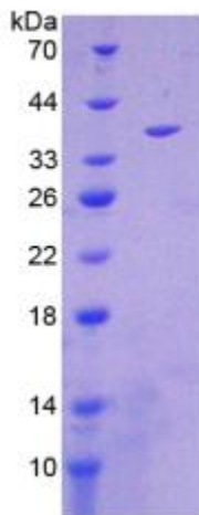
SDS-PAGE Image
