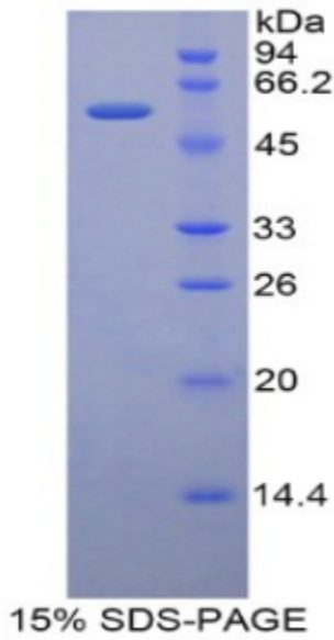
SDS-PAGE Image
