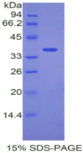
SDS-PAGE Image
