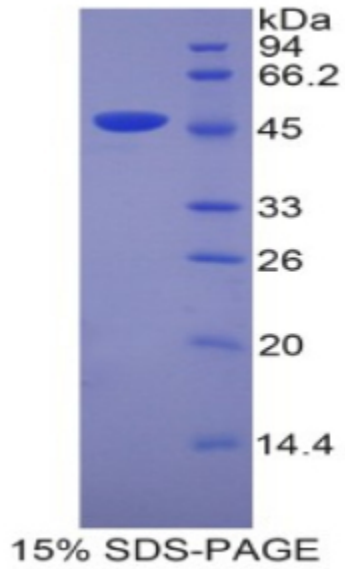
SDS-PAGE Image
