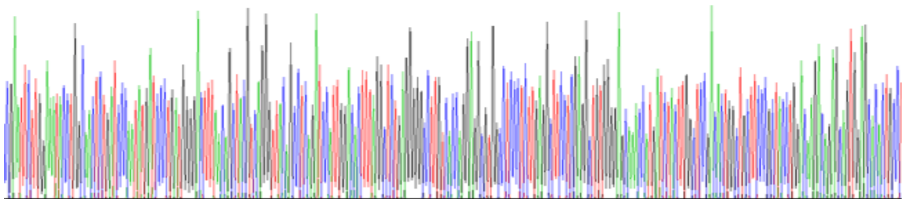
Figure. SDS-PAGE
