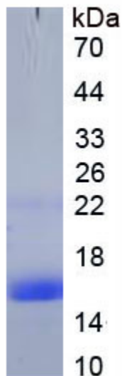
Figure. SDS-PAGE
