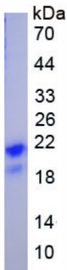
Figure. SDS-PAGE
