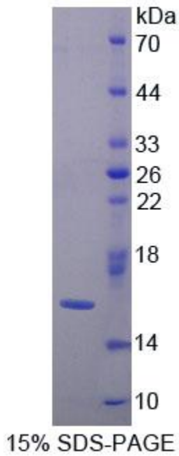
Figure. SDS-PAGE
